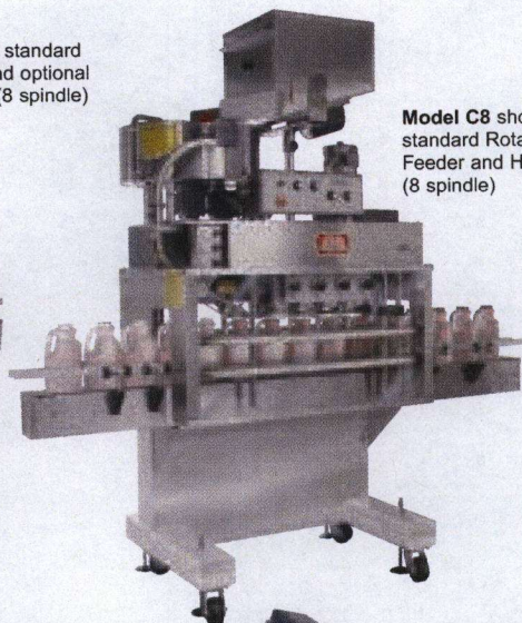
Model C8 shown with standard Rotary Cap Feeder, optional Bulk Elevator and optional Automatic Torque Monitor (8 spindle)
